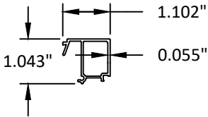
3 GLAZING BEAD 6063-T5
