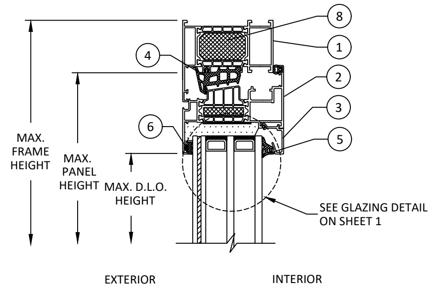
A 4 VERTICAL SECTION TYP. HEAD DETAIL
