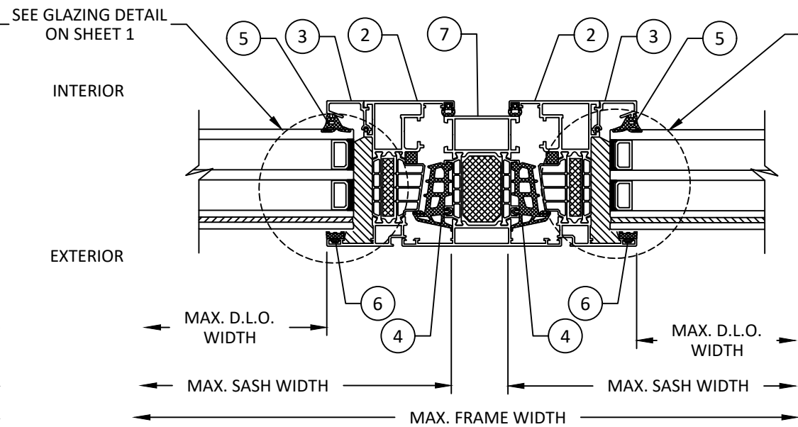
B HORIZONTAL SECTION 5 TYP. MULLION DETAIL
